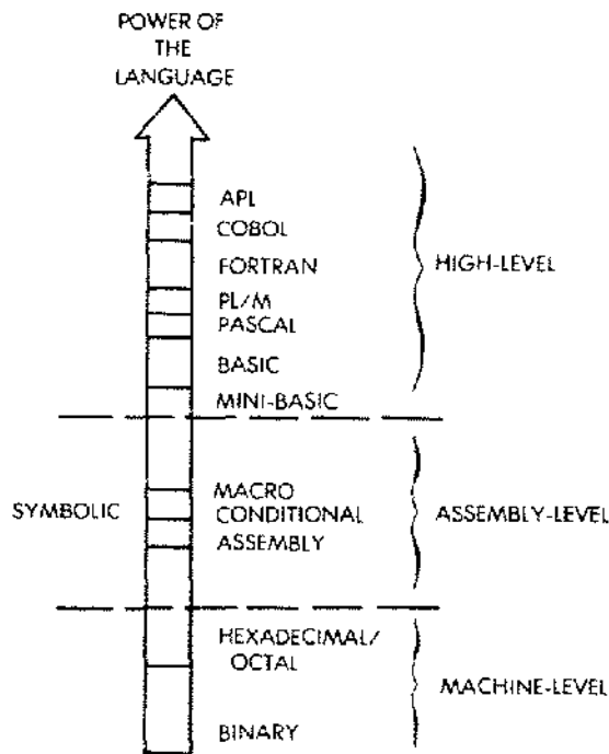
Fig. 10.1: Programming Levels
