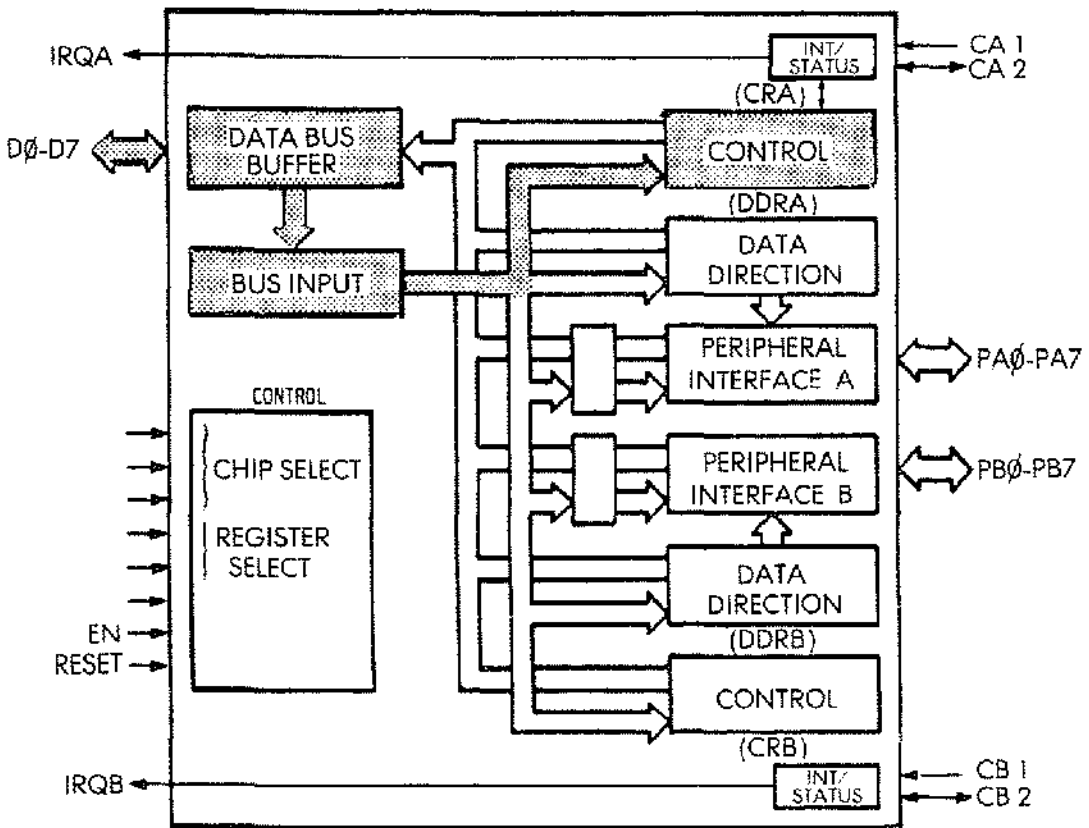
Fig. 7.2: Using a PIO-Load Control Register
