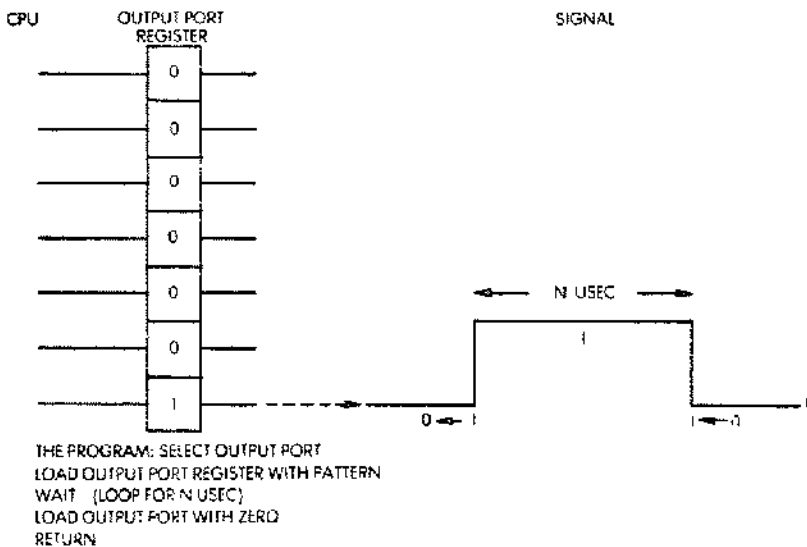
Fig. 6.2: A Programmed Pulse
