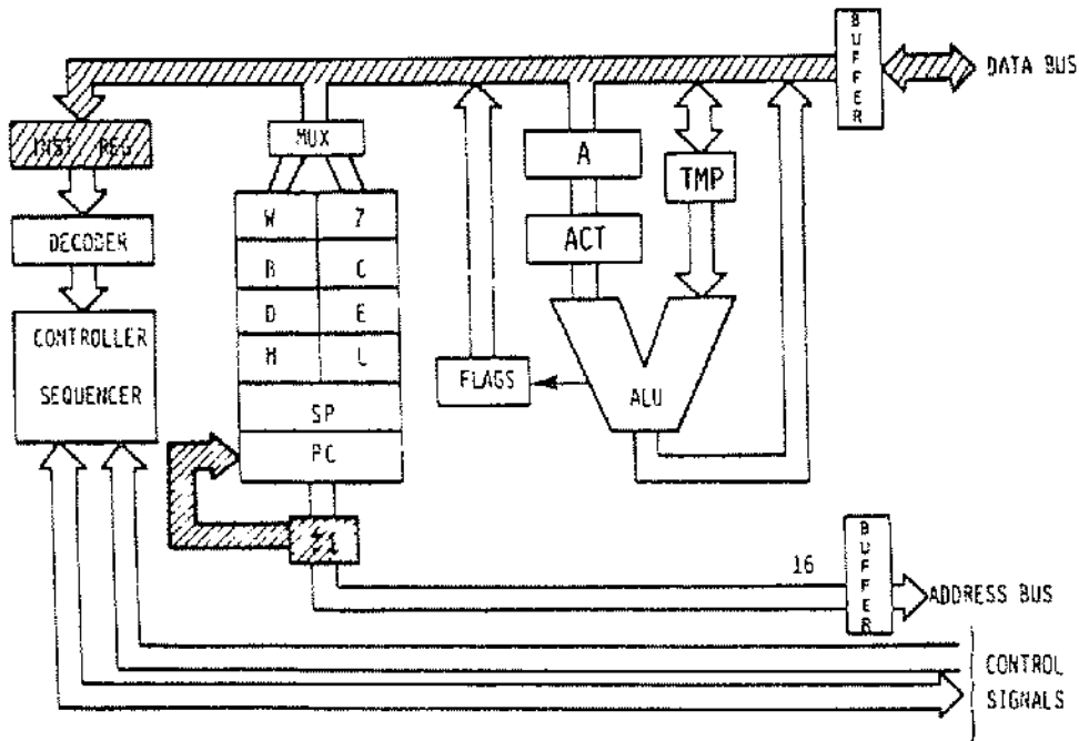
Fig 2.18: PC Is Incremented
