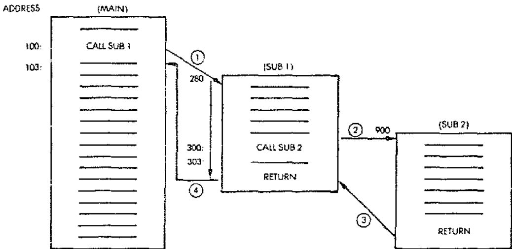
Fig. 3.37: The Subroutine Calls
