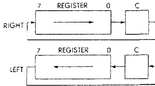
Fig. 4.11: Nine-Bit Rotation
