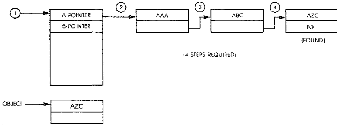
Fig. 9.26: Linked List—A Search
