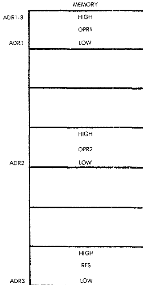
Fig. 3.8: A 32-Bit Addition
