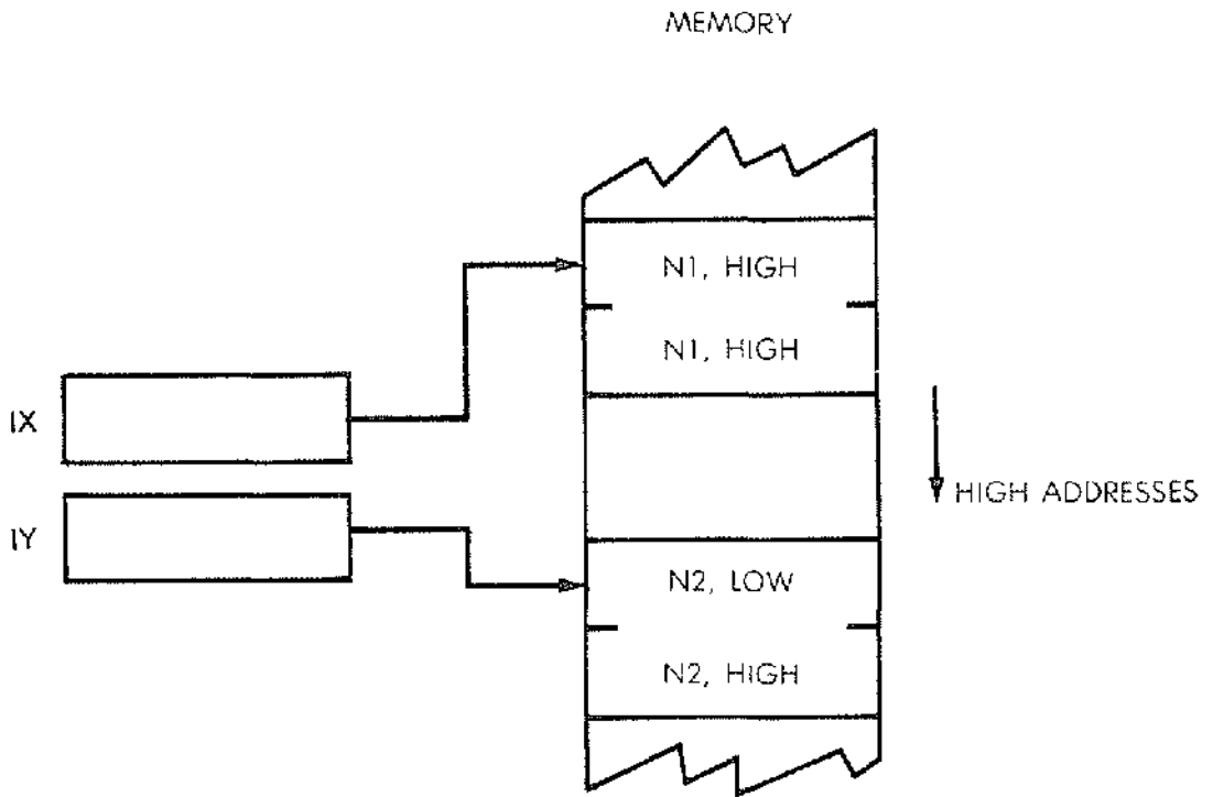
Fig. 8.4: Comparing Two Signed Numbers
