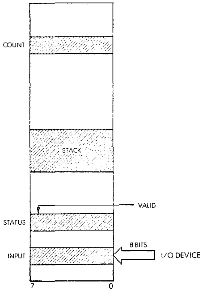
Fig. 6.4: Parallel Word Transfer - The Memory
