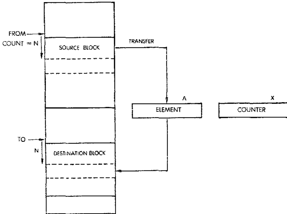
Fig. 5.10: Memory Organization for Block Transfer
