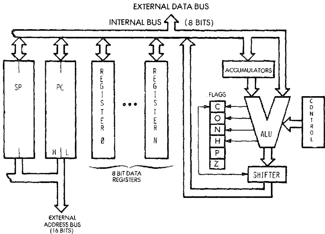
Fig. 2.2: "Standard" Microprocessor Architecture
