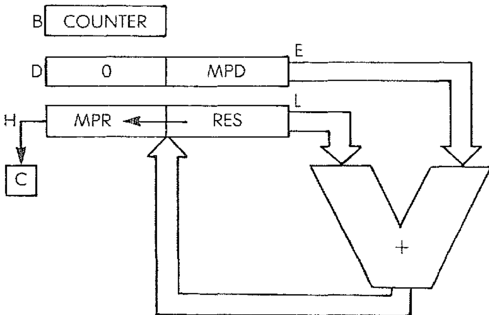
Fig. 3.25: Registers for Improved Multiply
