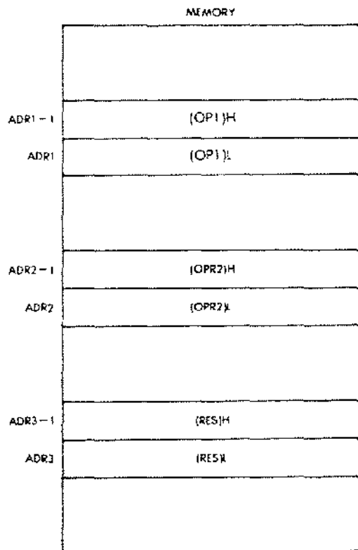
Fig. 3.5: 16-Bit Addition—The Operands
