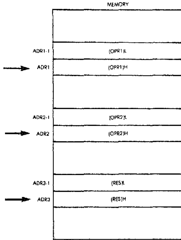
Fig. 3.7: Pointing to the High Byte
