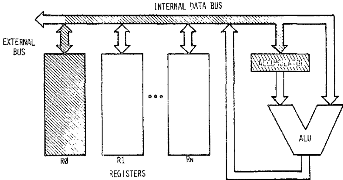
Fig. 2.9: Execution of an Addition—R0 into ACC
