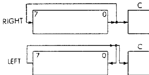
Fig. 4.12: Eight-Bit Rotation
