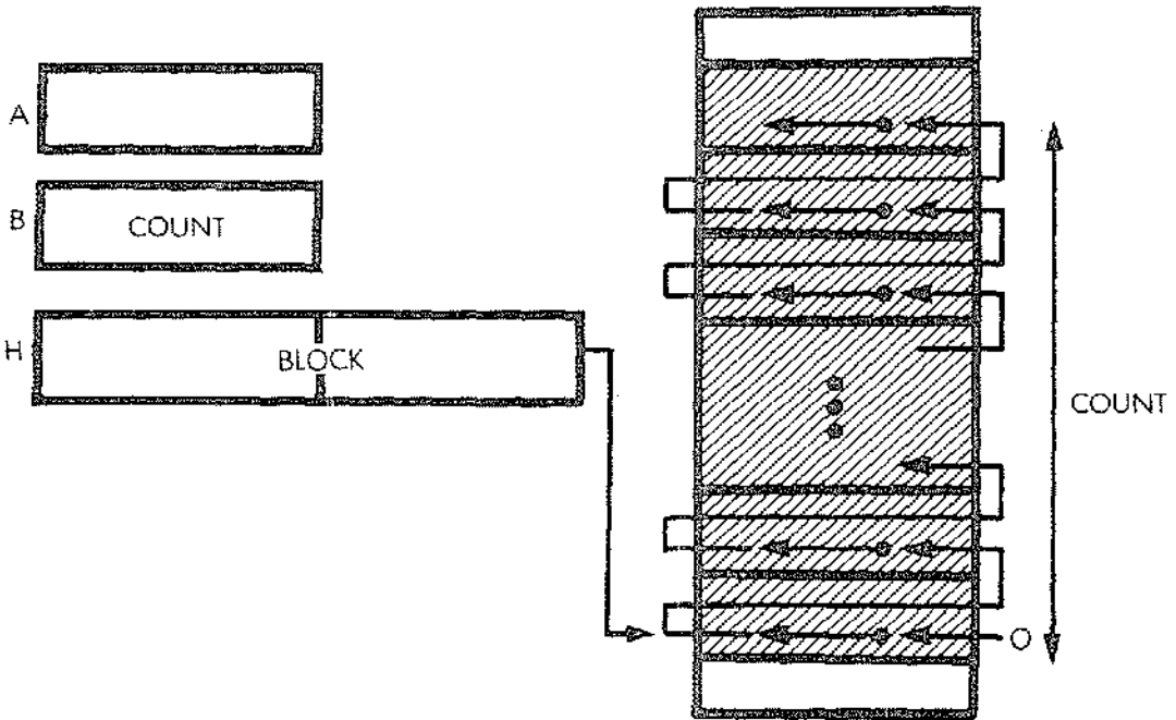
Fig. 8.3: BCD Block Transfer - The Memory
