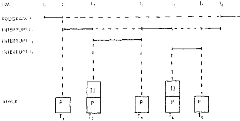
Fig. 6.33: Stack Contents During Multiple Interrupts
