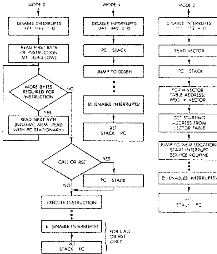
Fig. 6.26: Interrupt Modes
