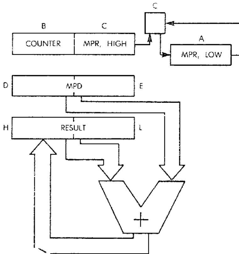
Fig. 3.27: 16 X 16 Multiply—The Registers
