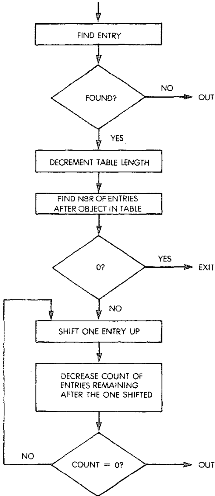
Fig. 9.15: Table Deletion Flowchart
