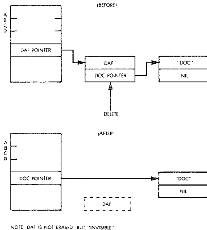
Fig. 9.28: Example of Deletion (Linked List)
