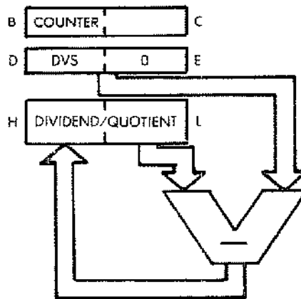
Fig. 3.31: 16 × 8 Division—The Registers
