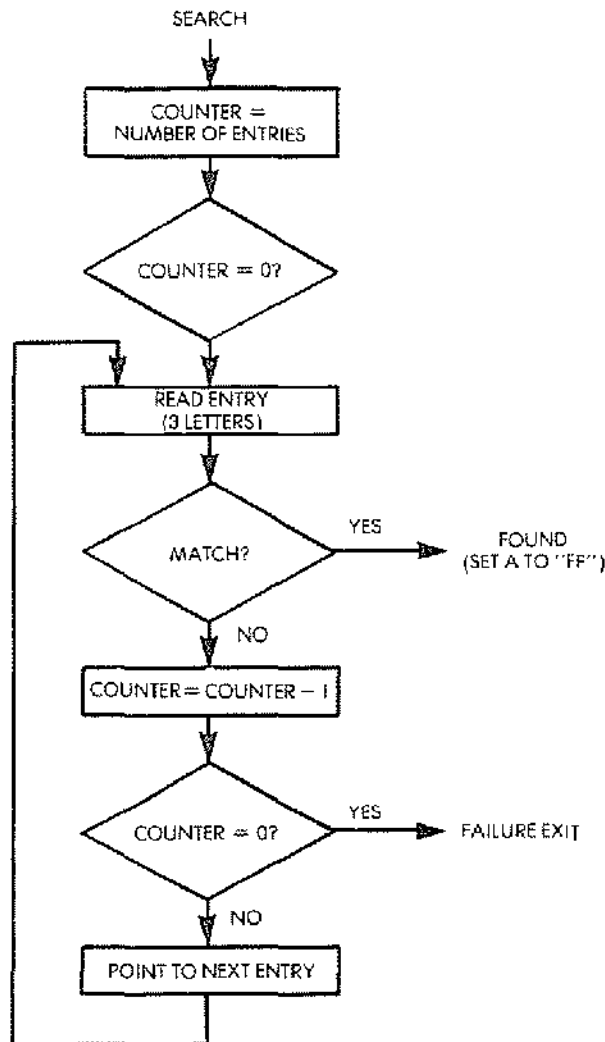
Fig. 9.12: Table Search Flowchart
