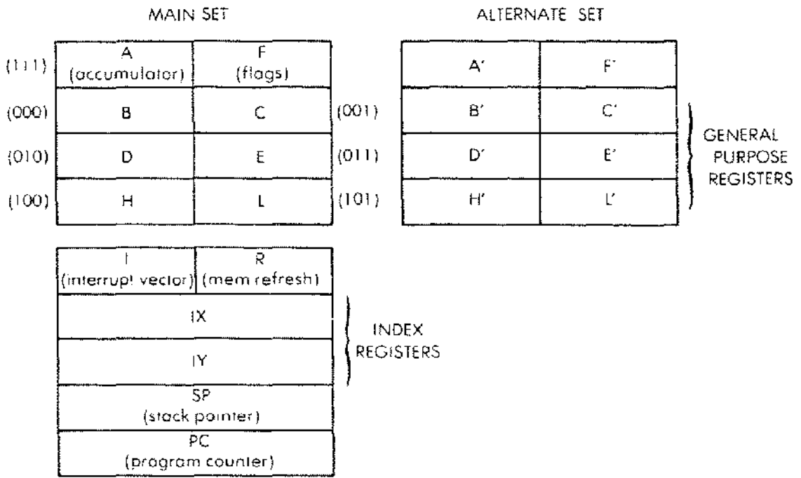
Fig. 3.0: The Z80 Registers
