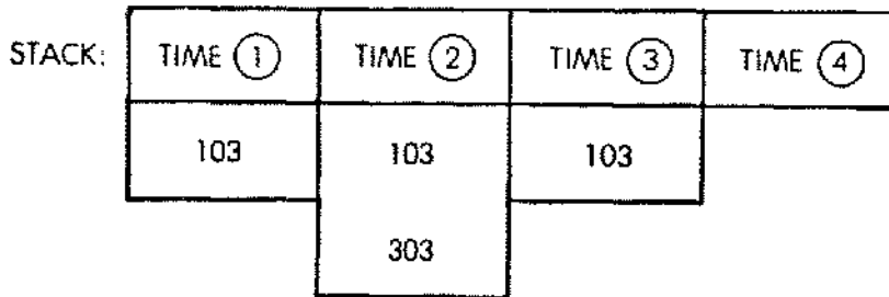
Fig. 3.38: Stack vs. Time
