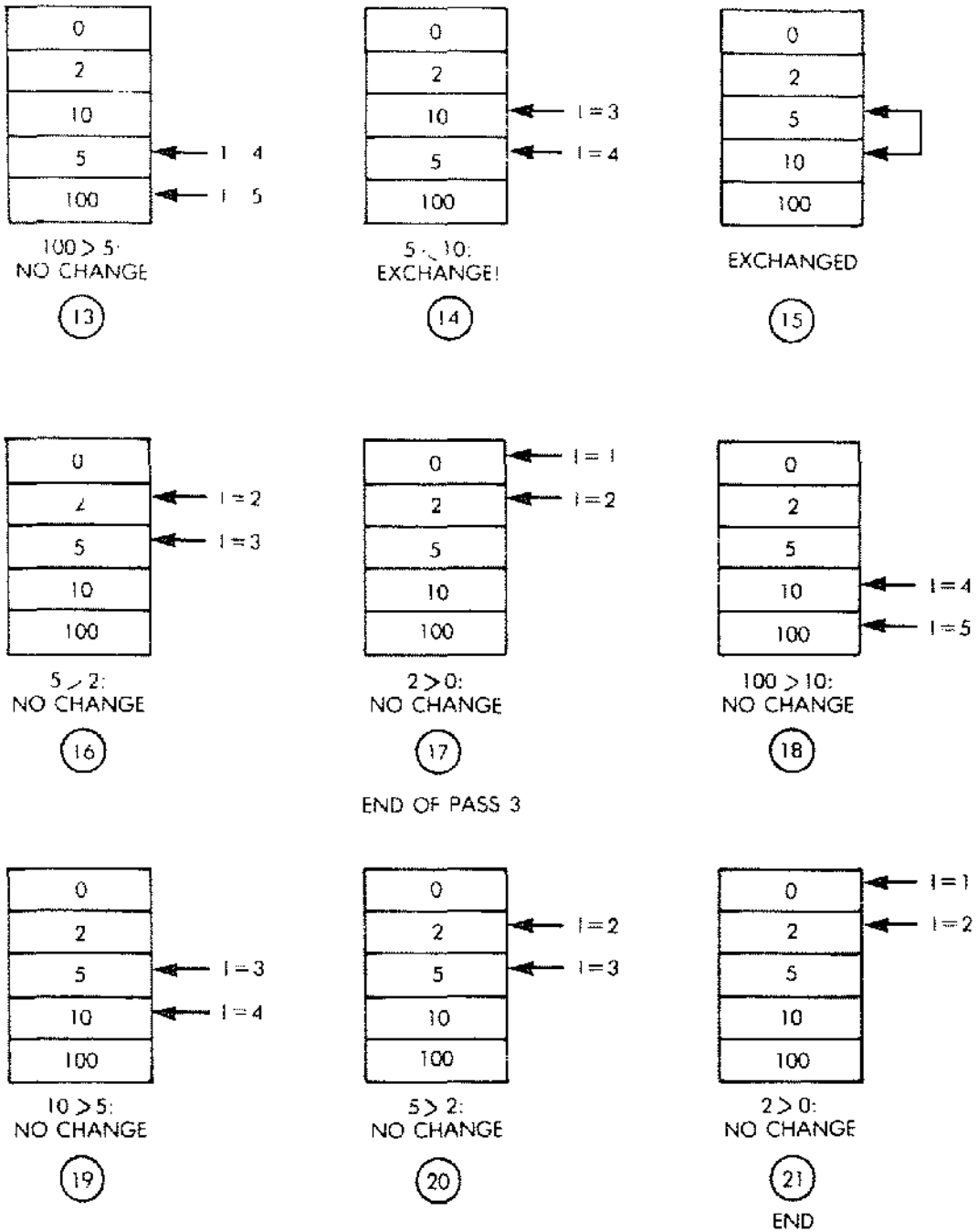
Fig. 8.6: Bubble-Sort Example: Phases 13 to 21
