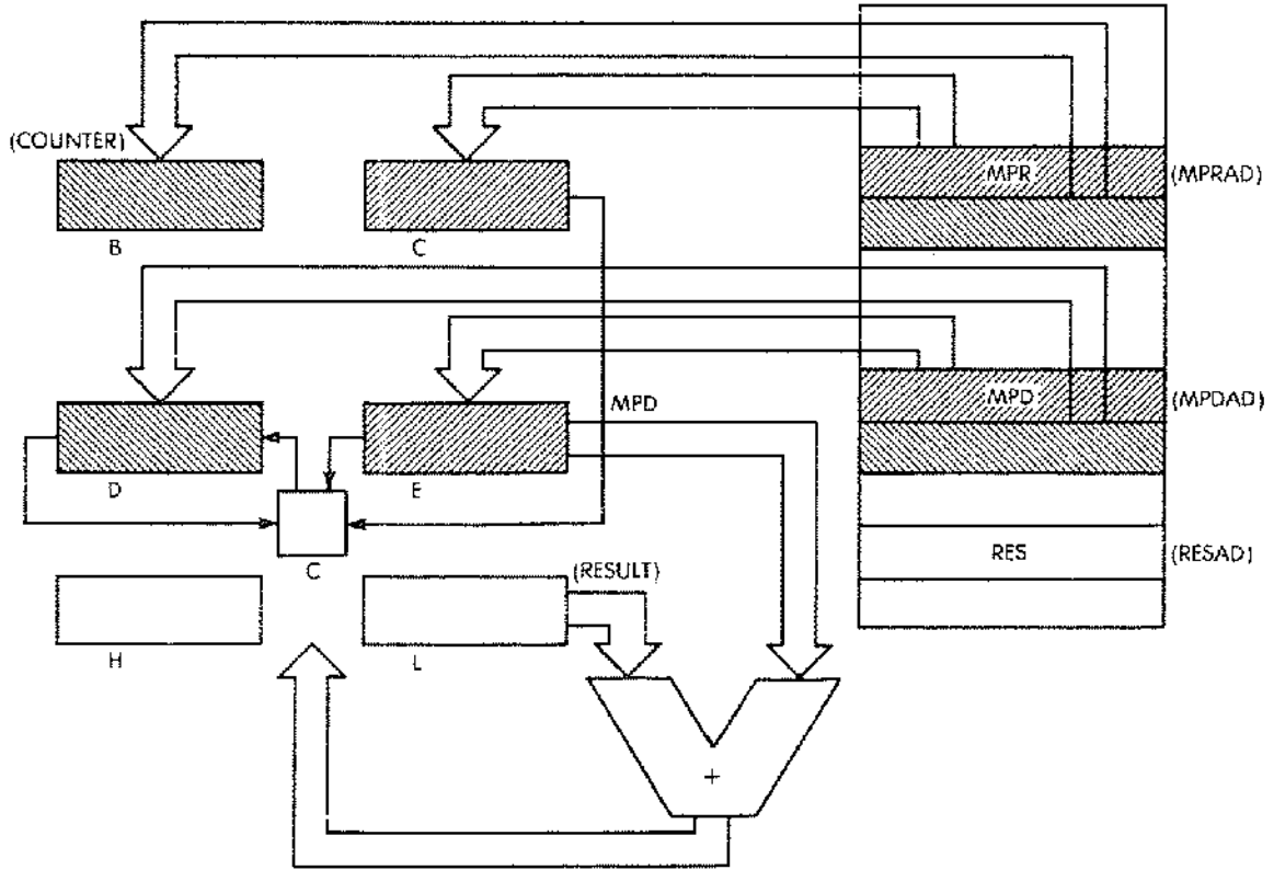
Fig 3.14: 8 × 8 Multiplication—The Registers
