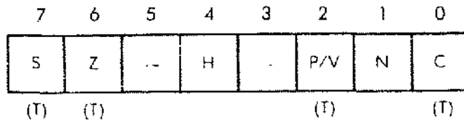
Fig. 4.16: The Flags Register
