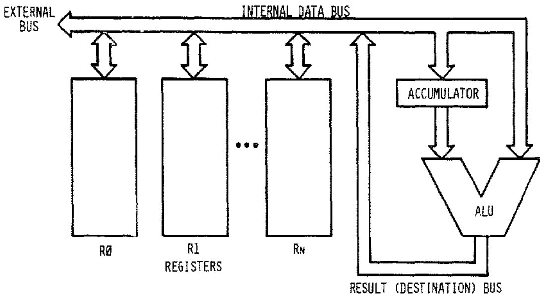
Fig. 2.8: Single-Bus Architecture
