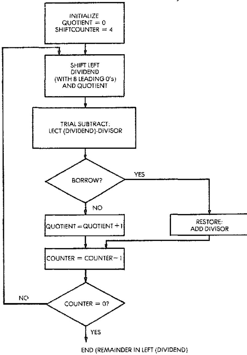
Fig. 3.30: 8-Bit Binary Division Flowchart
