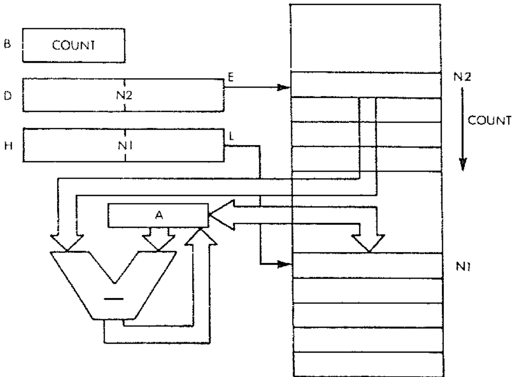
Fig. 3.11: Packed BCD Subtract: N1 \leftarrow N2 - N1
