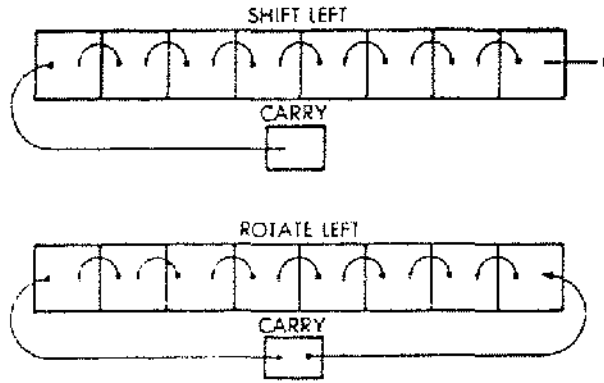
Fig. 4.9: Shift and Rotate
