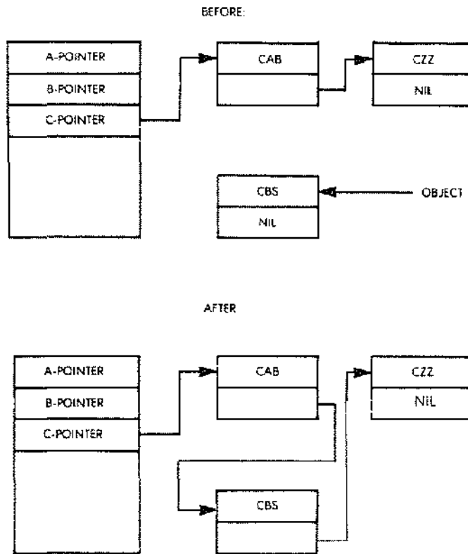
Fig. 9.27: Linked List: Example of Insertion
