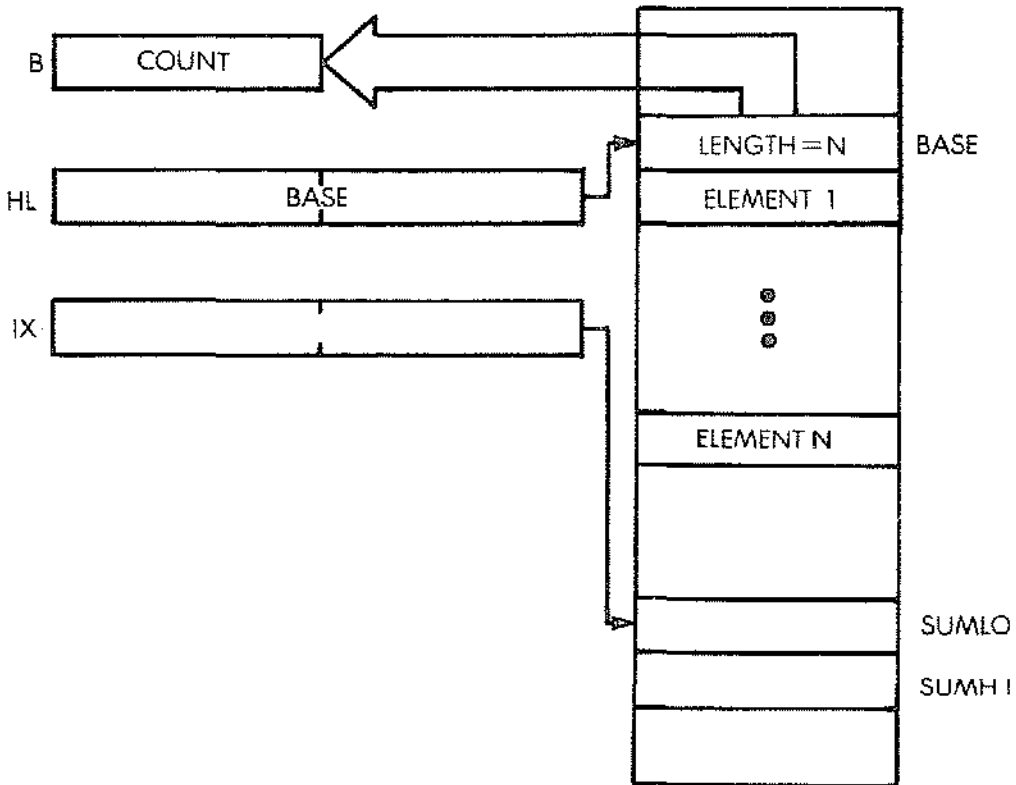
Fig. 8.2: Sum of N Elements
