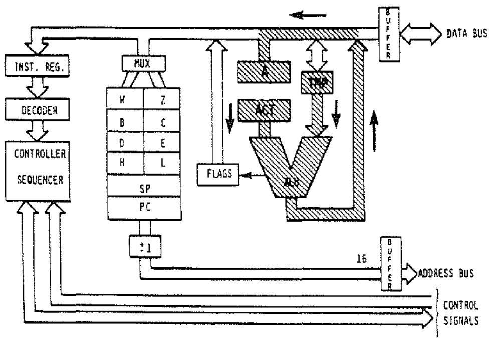
Fig. 2.24: End of ADD r
