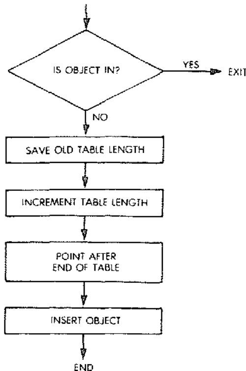
Fig. 9.13: Table Insertion Flowchart
