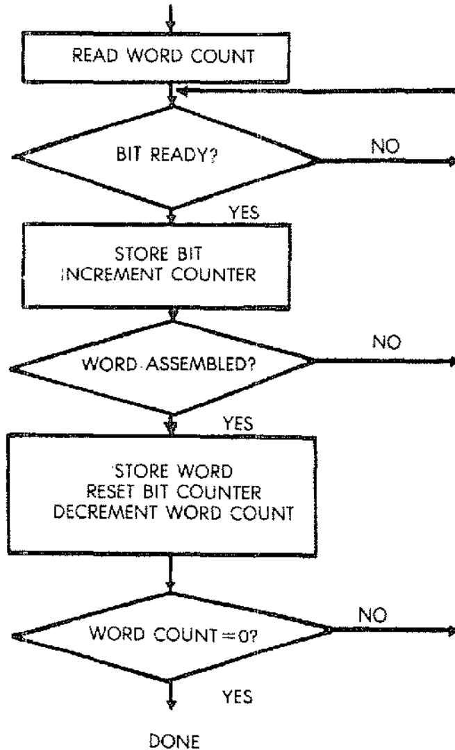
Fig. 6.6: Bit Serial Transfer—Flowchart
