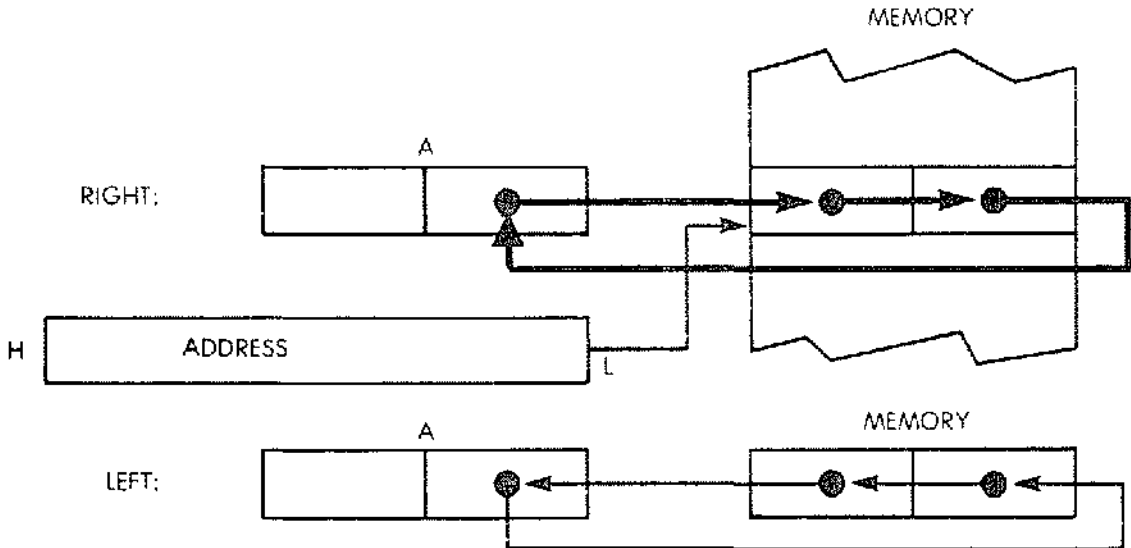
Fig. 4.13: Digit Rotate Instructions
