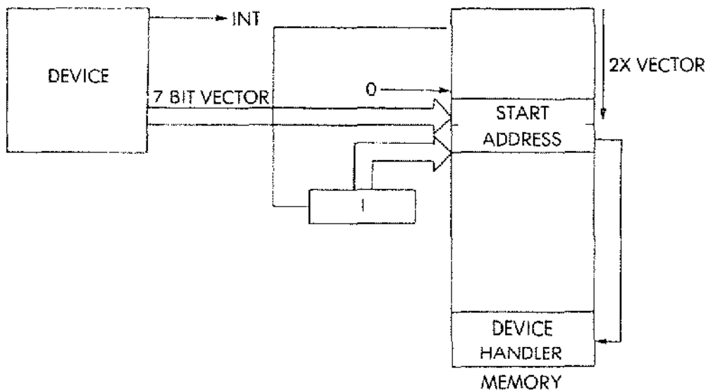
Fig. 6.29: Mode 2 Interrupt
