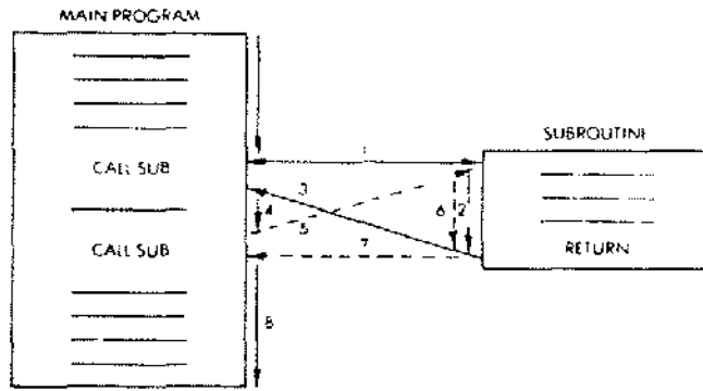
Fig. 3.35: Subroutine Calls
