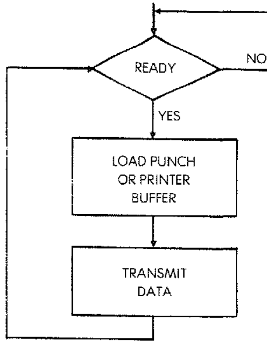
Fig. 6.21: Printing on a Punch or Printer
