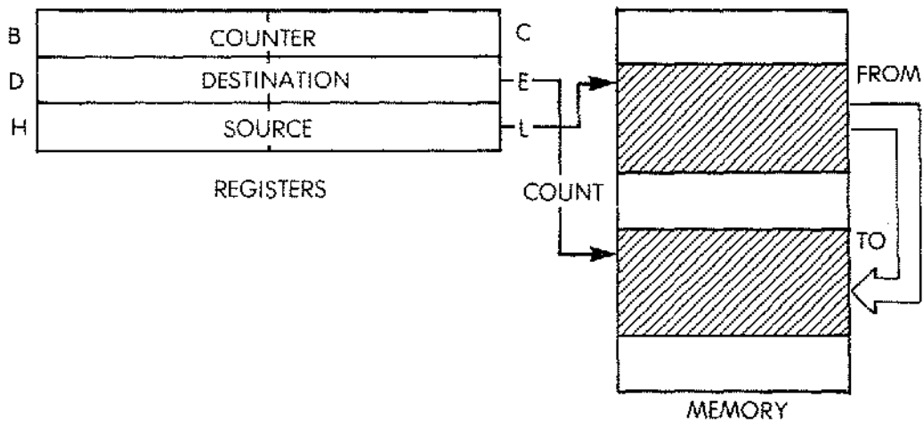
Fig. 5.8: A Block Transfer-Memory Map
