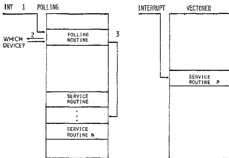
Fig. 6.31: Polled vs. Vectored Interrupt
