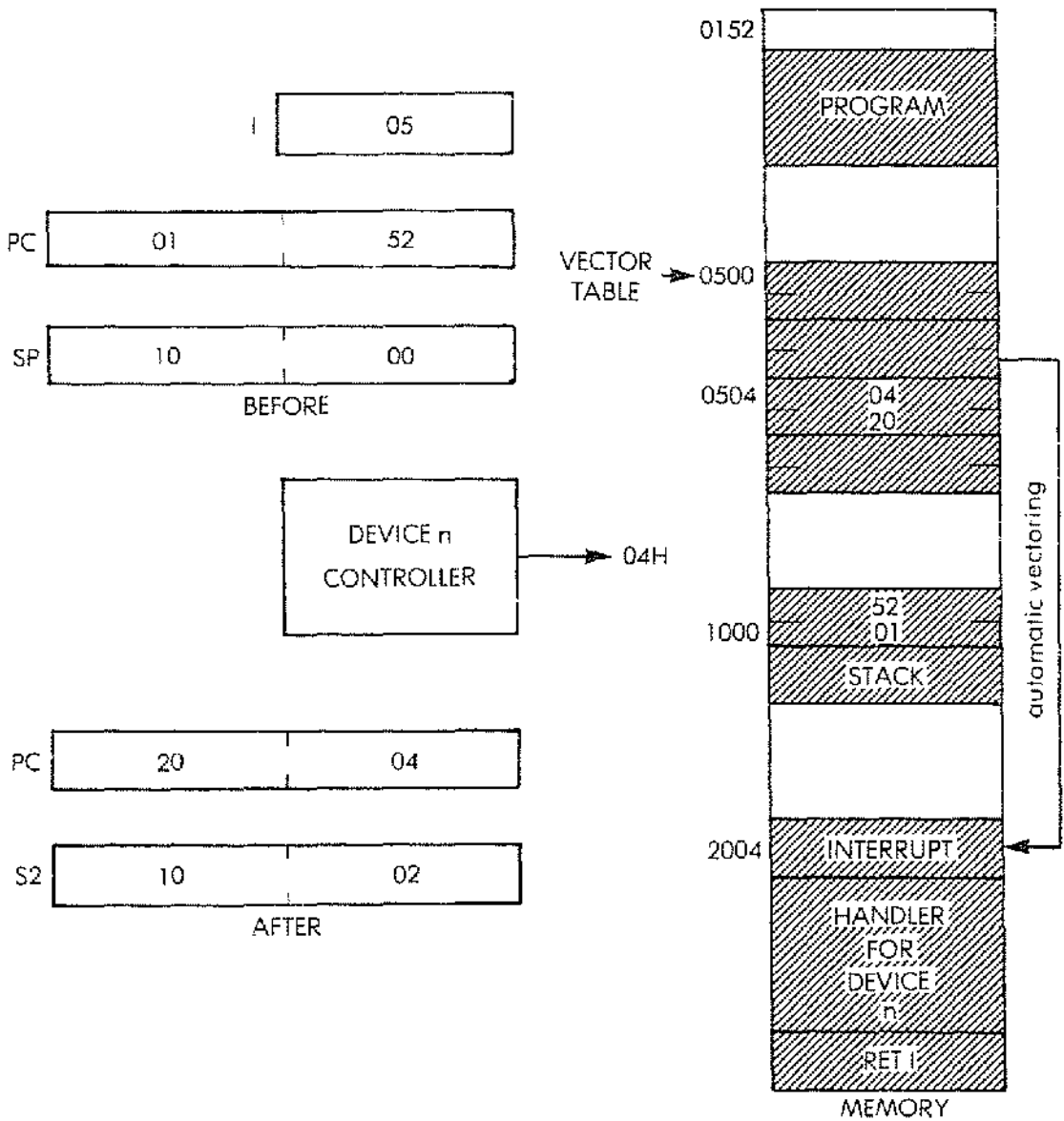
Fig. 6.30: Mode 2 - A Practical Example
