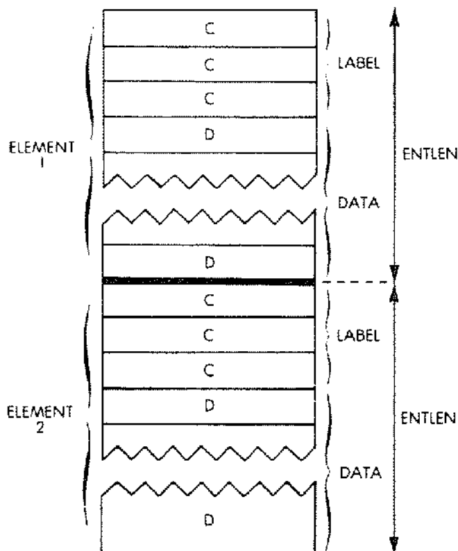
Fig 9.10: Typical List Entries in the Memory
