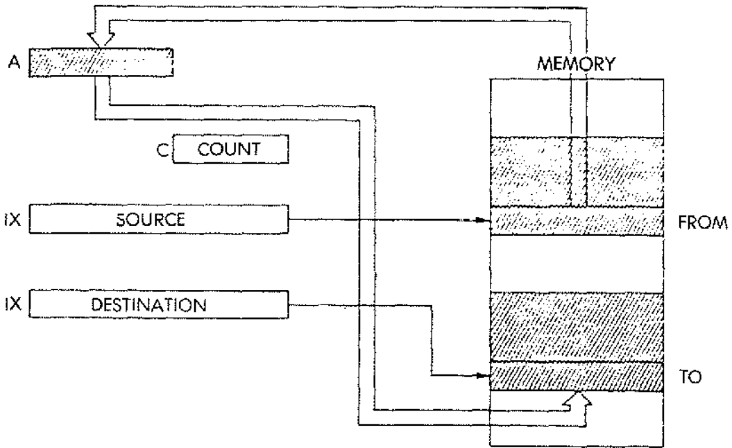
Fig. 5.7: Block Transfer: Initializing the Register
