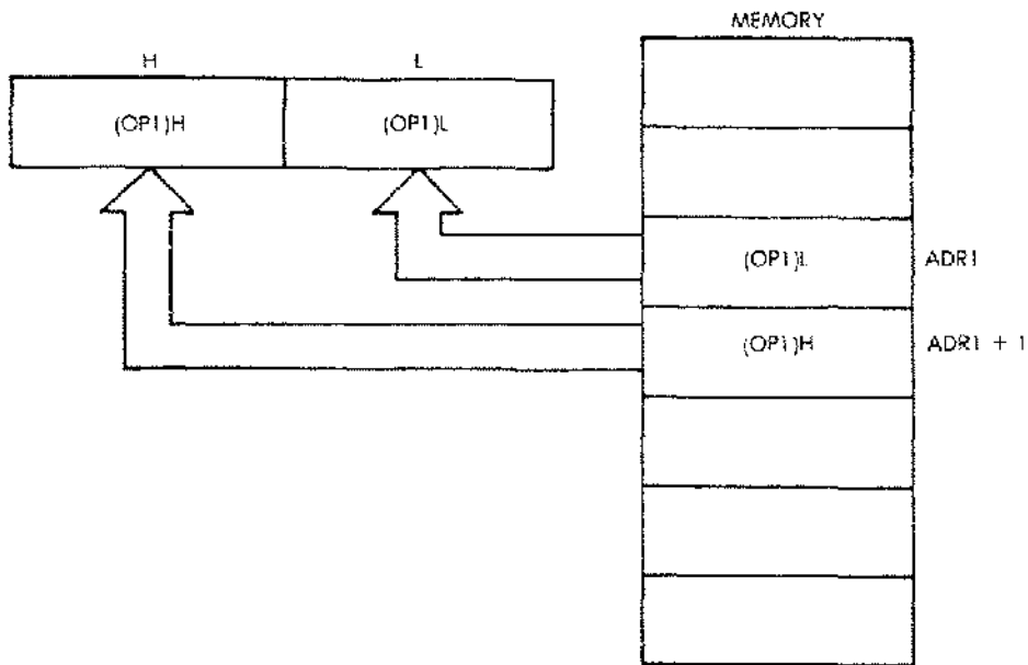
Fig. 3.9: 16-Bit Load — LD HL, (ADR1)
