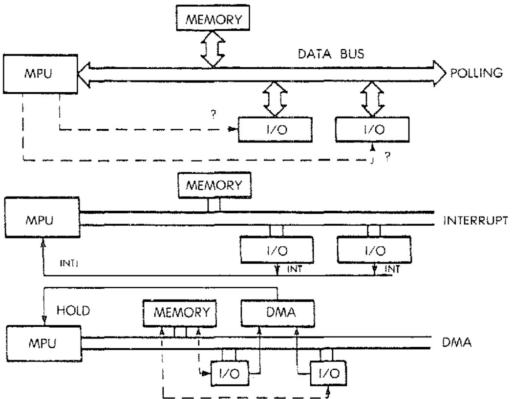
Fig. 6.18: Three Methods of I/O Control
