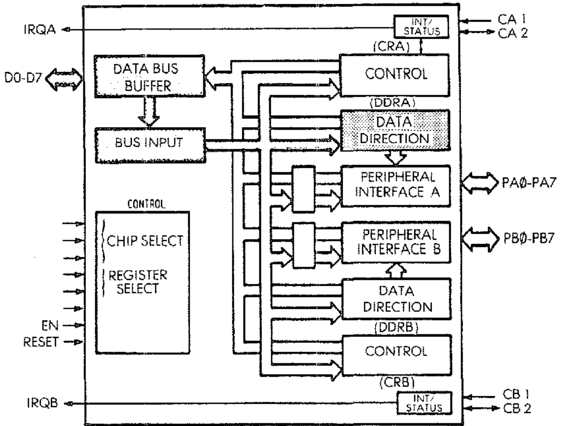
Fig. 7.3: Using a PIO-Load Data Direction
