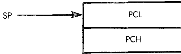
Fig. 6.22: Z80 Stack After Interruption
