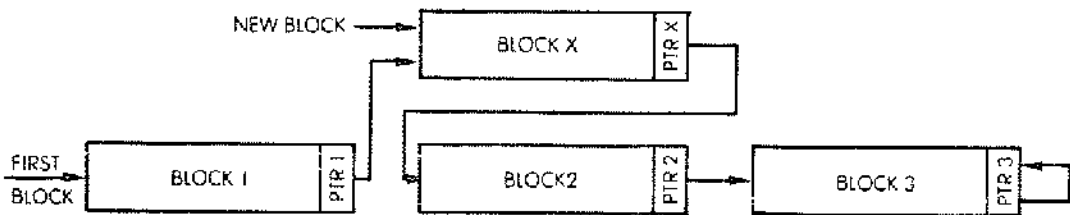
Fig. 9.4: Inserting a New Block
