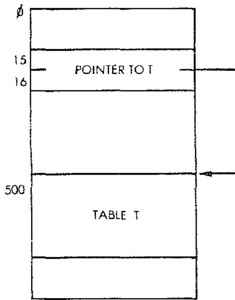
Fig. 9.1: An Indirection Pointer
