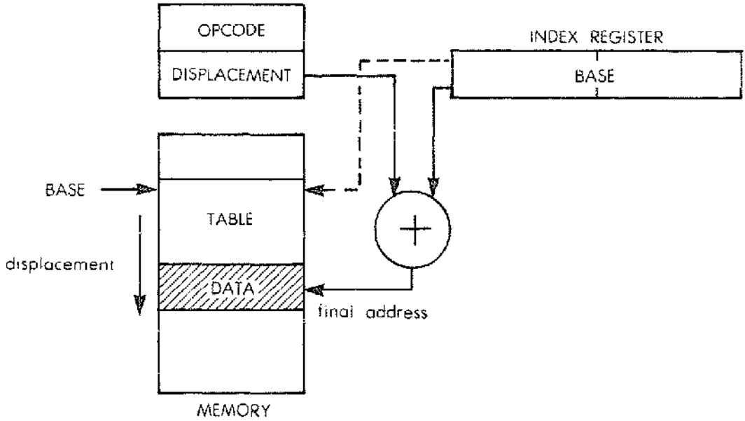
Fig. 5.2: Addressing (Pre-indexing)
