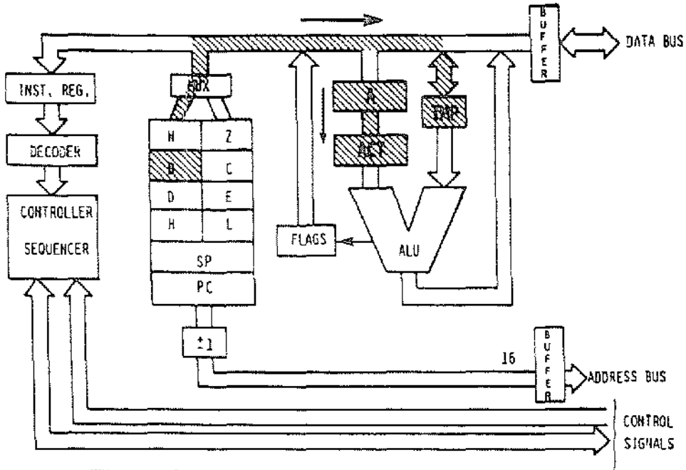
Fig. 2.23: Two Transfers Occur Simultaneously
