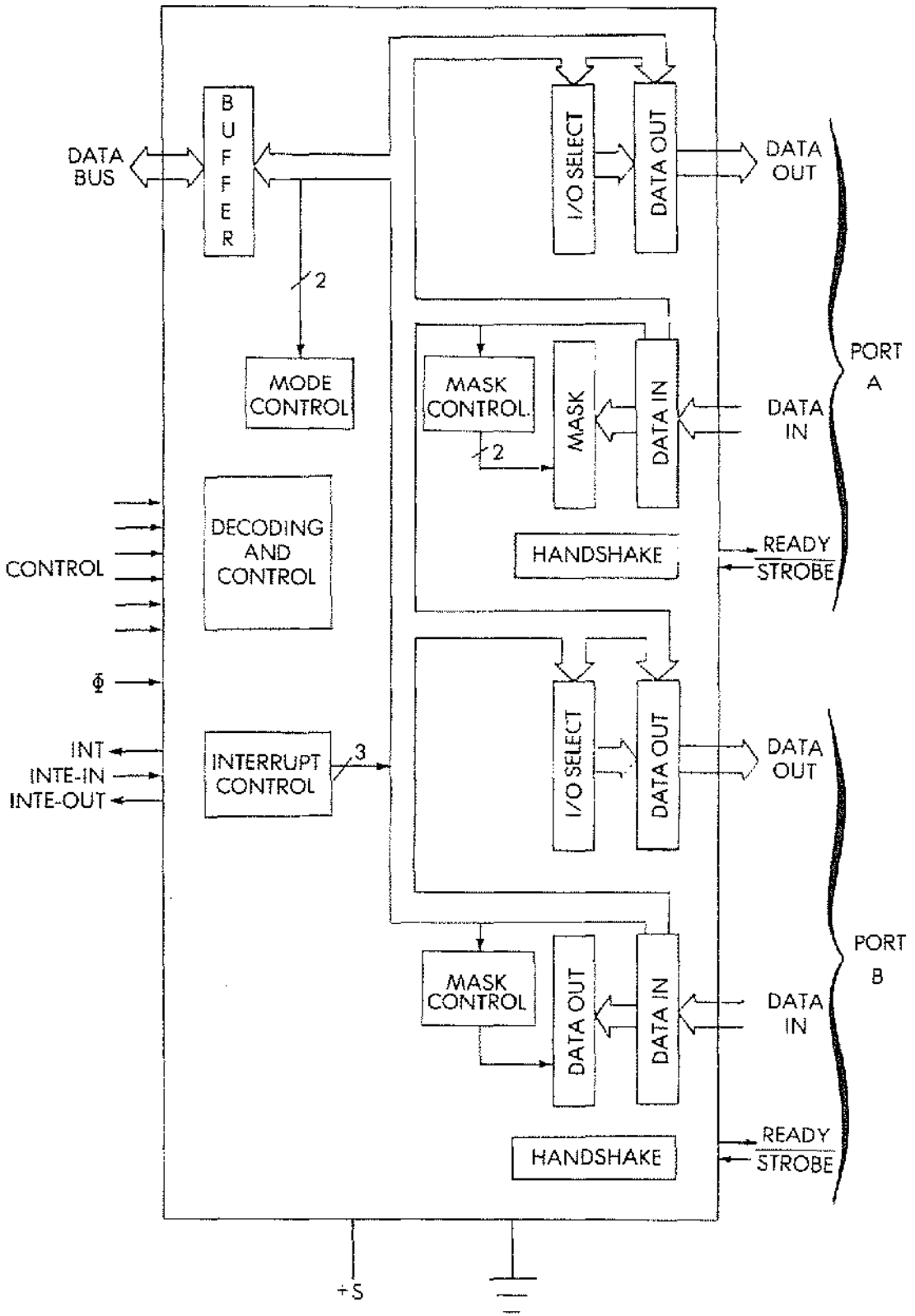
Fig. 7.7: Z80 PIO Block Diagram
