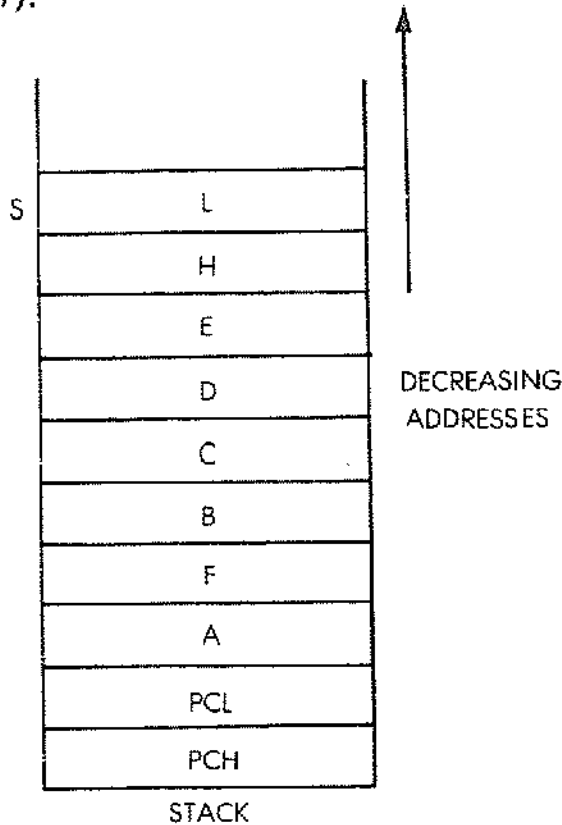
Fig. 6.27: Saving the Registers
