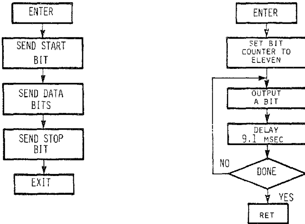
Fig. 6.16: Teletype Output
