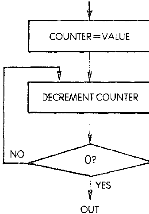
Fig. 6.3: Basic Delay Flowchart
