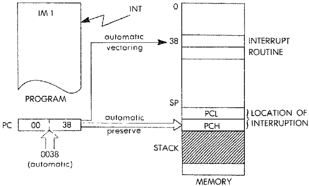
Fig. 6.28: Mode 1 Interrupt
