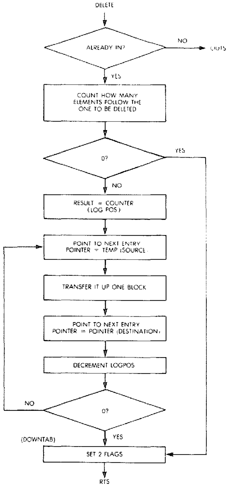
Fig. 9.22: Deletion Flowchart (Alphabetic List)
