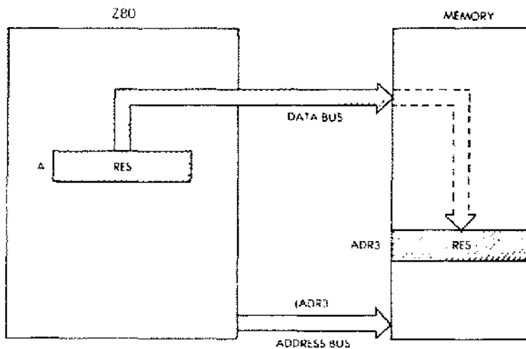
Fig. 3.4: LD (ADR3), A (Save Accumulator in Memory)
