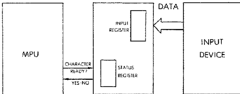
Fig. 6.8a: Handshaking (Input)
