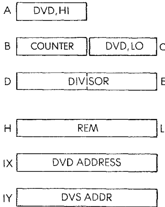
Fig. 3.34: Non-Restoring Divisor—The Registers
