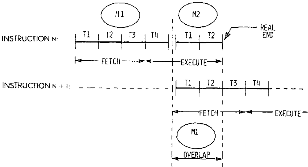
Fig. 2.25: FETCH-EXECUTE Overlap during T1-T2
