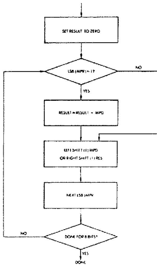
Fig. 3.12: The Basic Multiplication Algorithm—Flowchart
