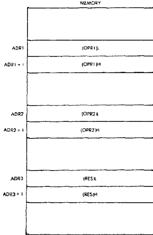
Fig. 3.6: Storing Operands in Reverse Order
