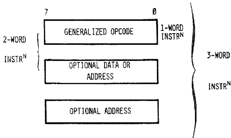
Fig. 2.15 Typical Instruction Formats
