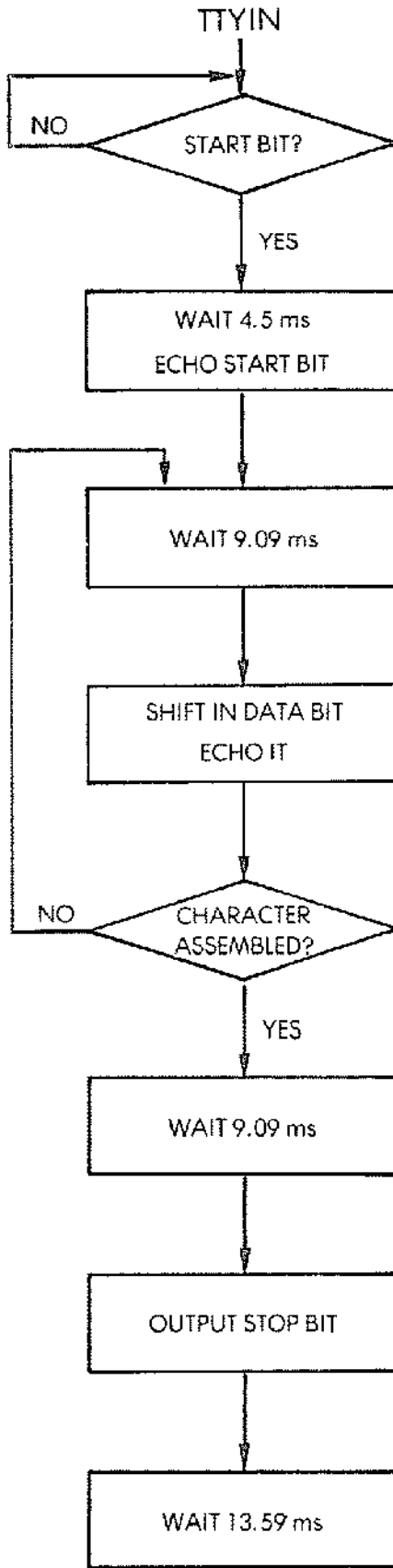
Fig. 6.13: TTY Input with Echo
