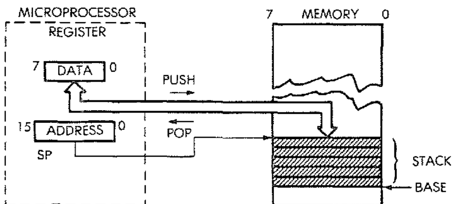
Fig. 2.5: The Two-Stack Manipulation Instructions
