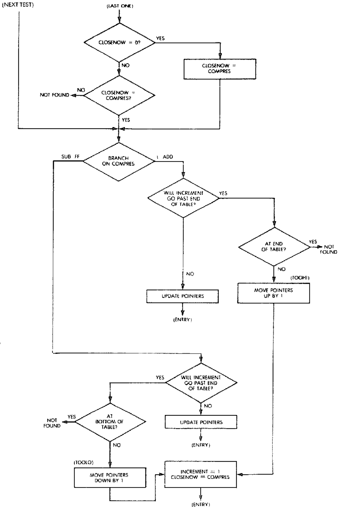
Fig. 9.18: Binary Search Flowchart (cont.)
