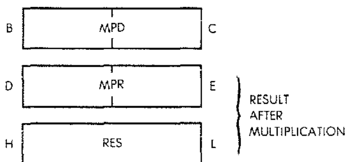
Fig. 3.29: 16 × 16 Multiply with 32-Bit Result
