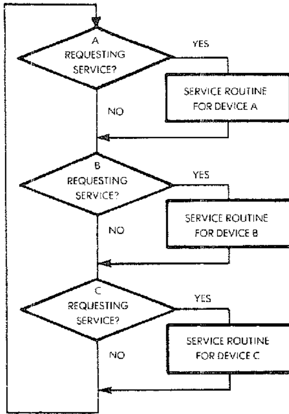
Fig. 6.19: Polling Loop Flowchart
