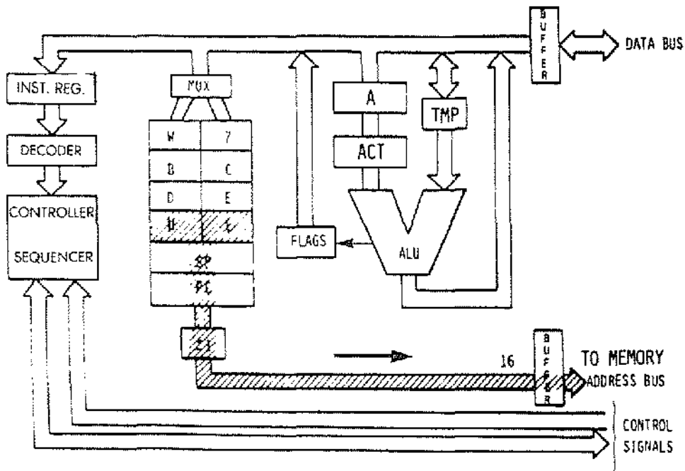
Fig. 2.28: Transfer Contents of HL to Address Bus
