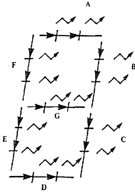
Fig. 6.10: Seven-Segment LED
