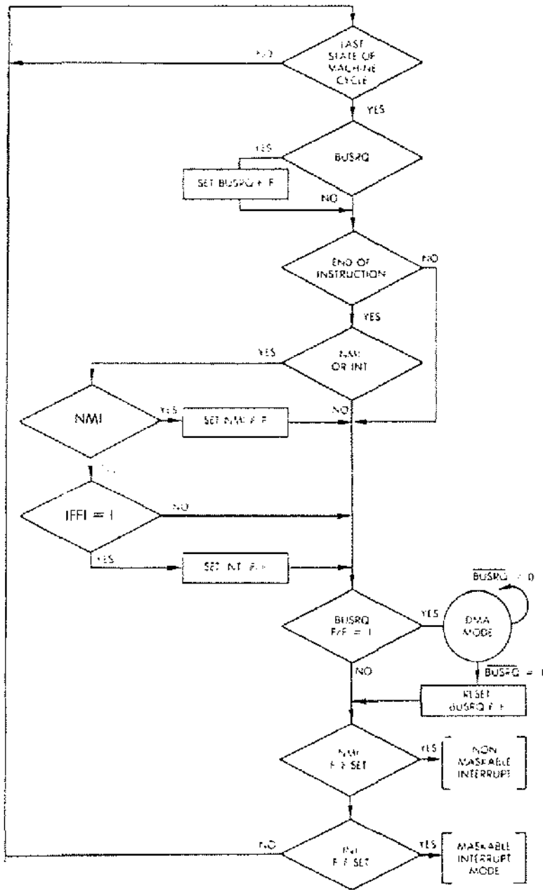
Fig. 6.24: Interrupt Sequence
