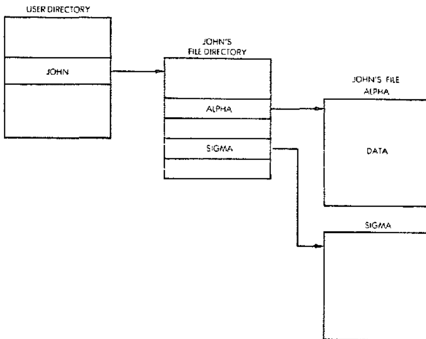
Fig. 9.2: A Directory Structure
