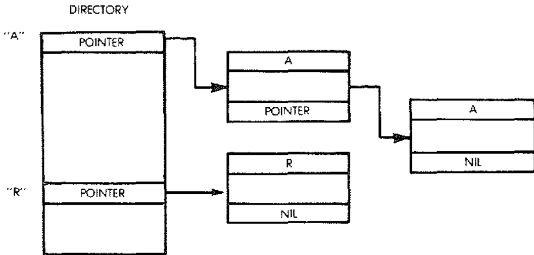
Fig. 9.25: Linked List Structure
