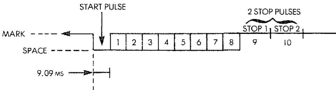
Fig. 6.12: Format of a Teletype Word
