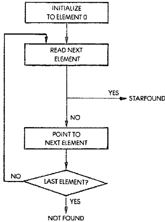
Fig. 5.6: Character Search Flowchart
