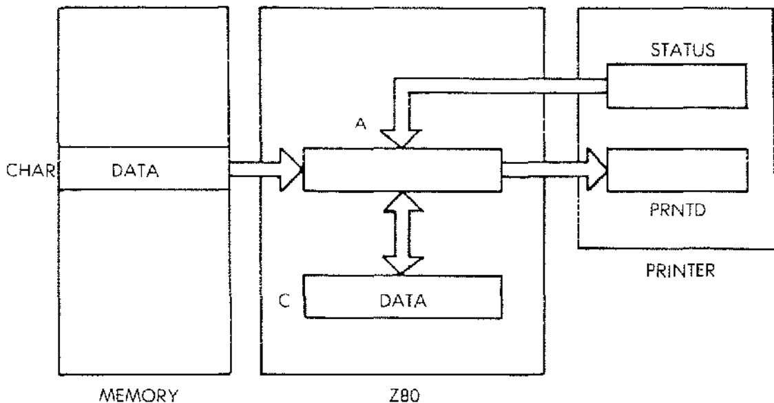
Fig. 6.9: Printer—Data Paths
