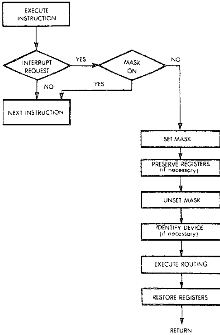
Fig. 6.34: Interrupt Logic
