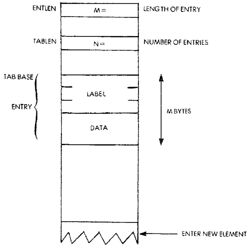
Fig. 9.9: The Table Structure
