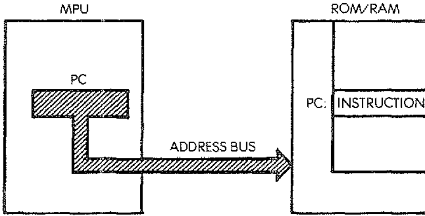
Fig. 2.6: Fetching an Instruction from the Memory
