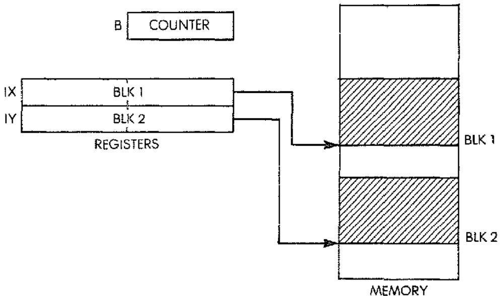
Fig. 5.9: Adding Two Blocks: BLK1 = BLK1 + BLK2
