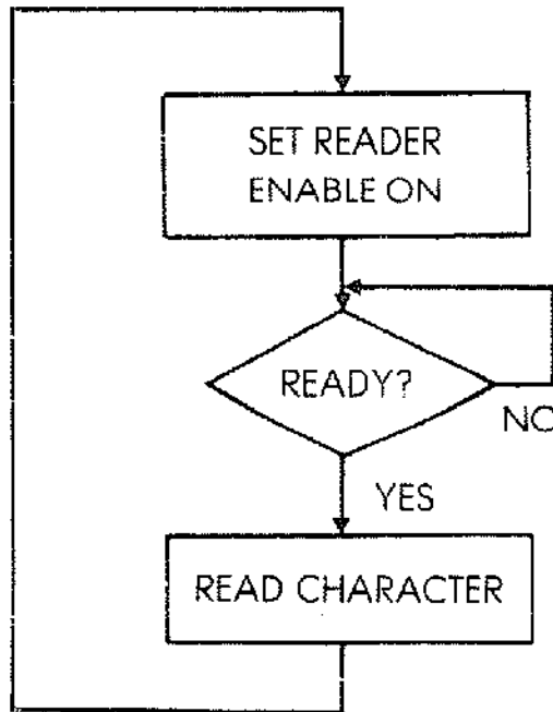
Fig. 6.20: Reading from a Paper-Tape Reader
