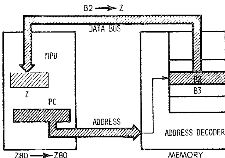
Fig. 2.32: Second Byte of Instruction Goes into Z
