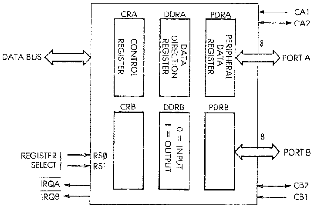
Fig. 7.1: Typical PIO
