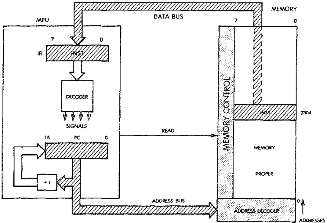
Fig. 2.7: Automatic Sequencing
