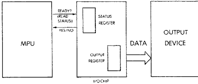
Fig. 6.8: Handshaking (Output)
