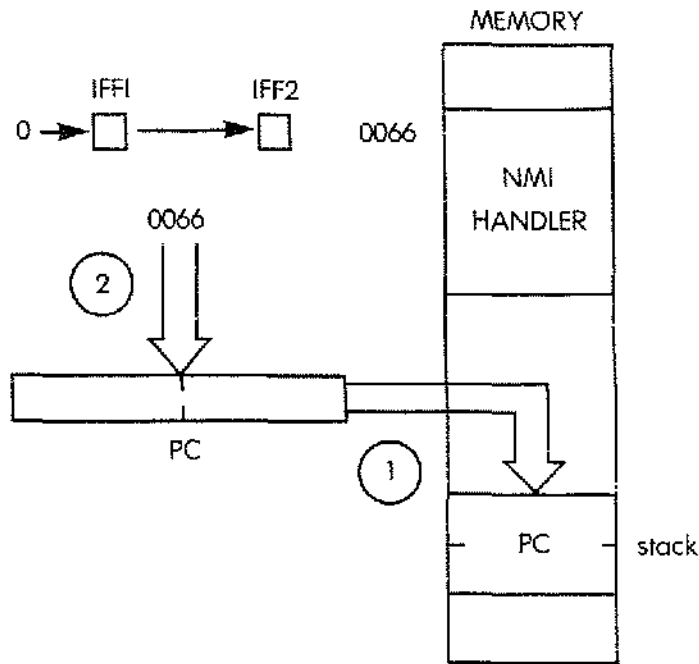
Fig. 6.25: NMI Forces Automatic Vectoring
